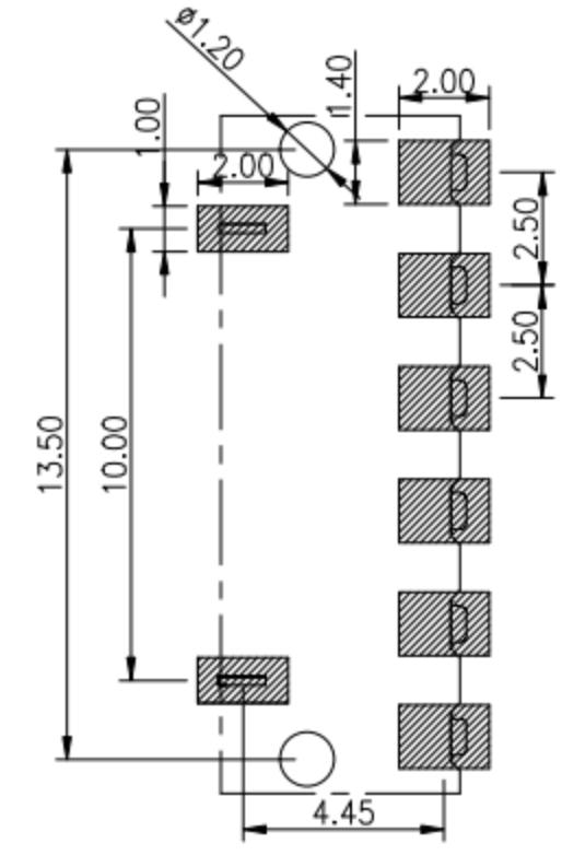
RECOMMENDED PCB LAYOUT TOP VIEW (.XX±0.05)
